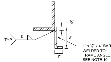
TAB DETAIL
