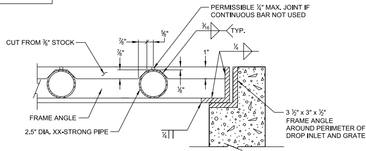
DETAIL A
