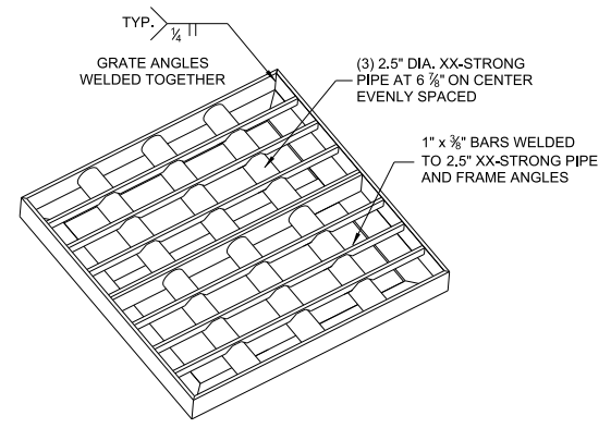
GRATE DETAIL
